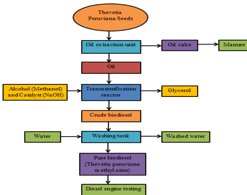
Figure. 1: Flow chart of biodiesel production [5]
