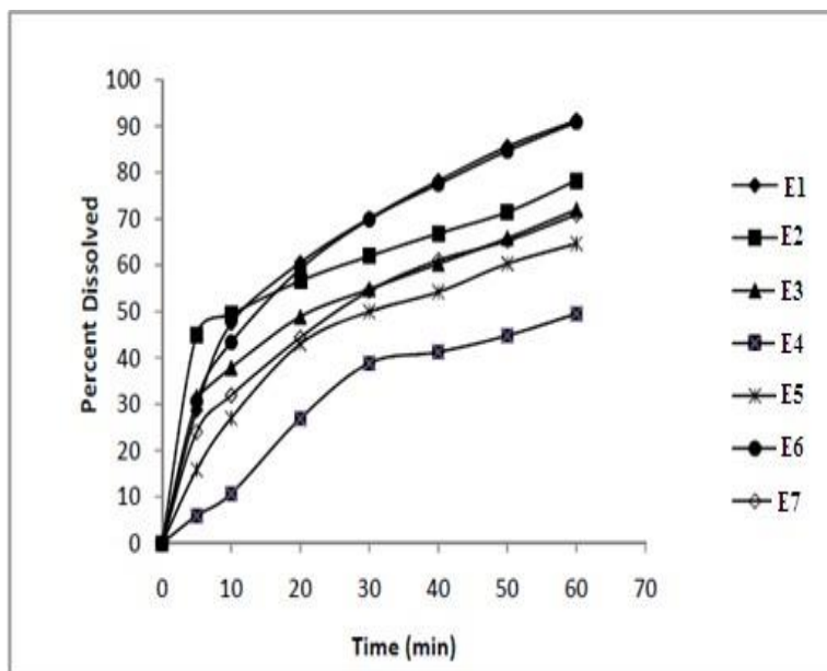
Fig. 2: Release of Tablets Manufactured with Multiple Granulators
