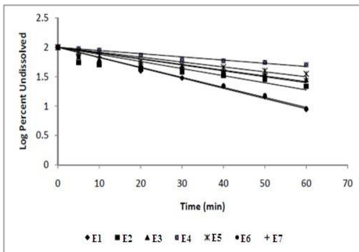
Figure. 3: Logarithmic Release of Tablets Manufactured with Multiple Granulating Agents
